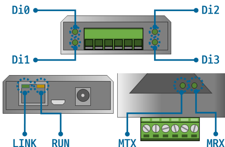
Схема 1-10 4 LED
