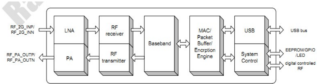
Figure 1: System Block Diagram of GWF-3S03 5.0V WLAN adapter
